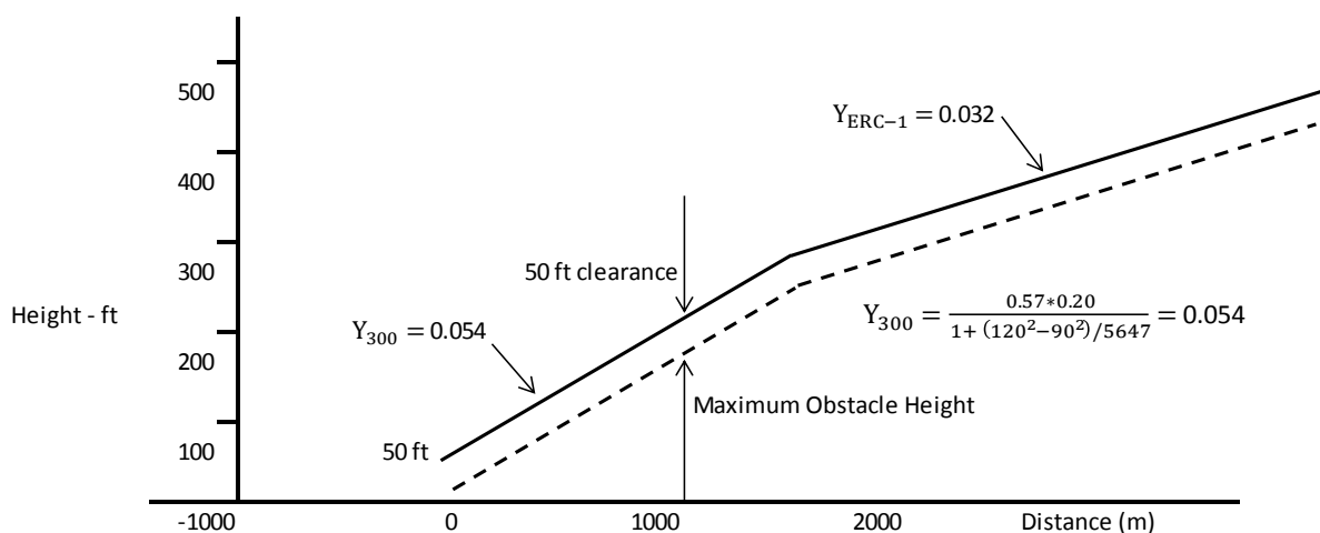
Figure 1: Assumed engine failure height 300 ft
