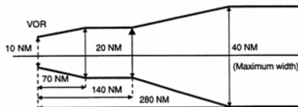
Figure 1: Corridor width from a VOR station
